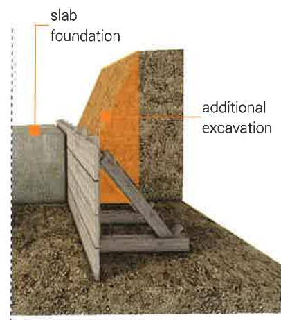
excavation - traditional formwork
